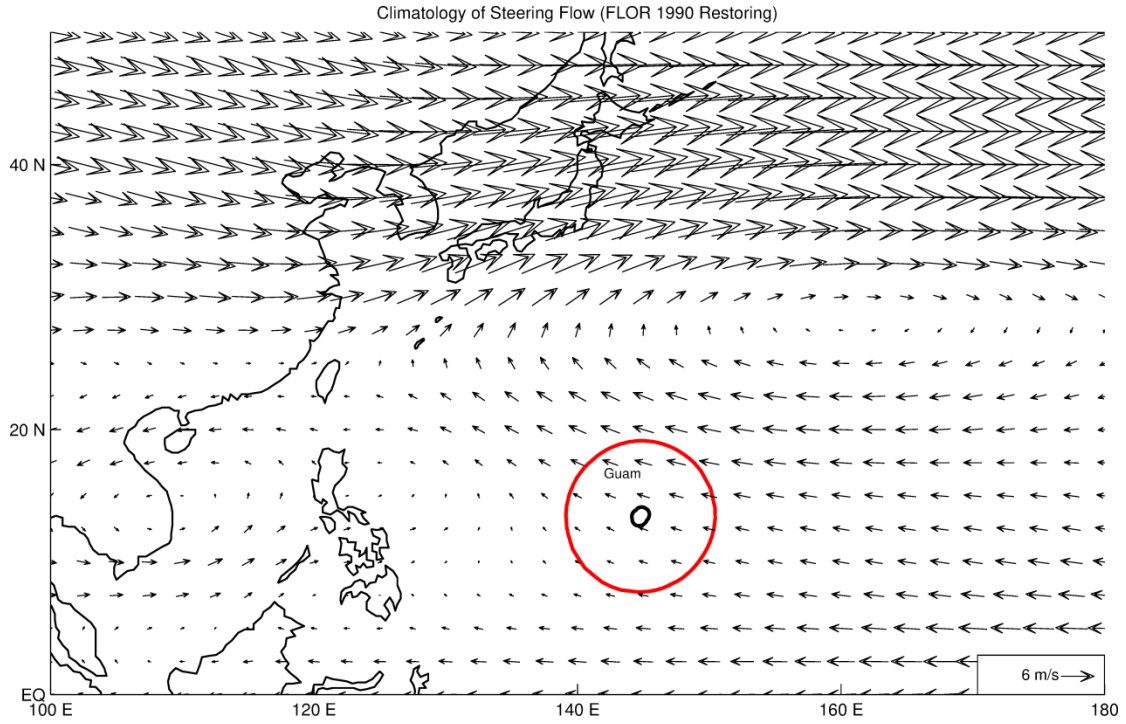
Figure S1 Climatology of steering flow (vector, unit: \text{ms}^{-1} ) in SST-nudging experiments with FLOR 1990. The black polygon and the outside circle denote Guam and its 500-km buffer zone which is used to define GuamTC.
