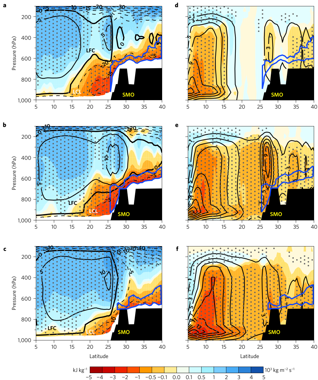
Figure 3 | CO 2 -induced warming strengthens convective inhibition and weakens convection over land. a–c , Difference in June (a), July–August (b), and September–October (c) mean buoyancy ( \text{kJ kg}^{-1} ) between doubled CO 2 and control FLOR-FA simulations (colour shading; see Methods for details on buoyancy calculations). Stippling denotes statistical significance, black lines denote climatological values of buoyancy (negative values are dashed), LFC the level of free convection (zero buoyancy), and LCL the lifted condensation level. Buoyancy values below the LCL are not shown because the relationship between buoyancy and moist static energy does not hold for an unsaturated parcel. d–f , As in a–c , but for the cumulus convective mass flux ( 10^3 \text{ kg m}^{-2} \text{ s}^{-1} ). The vertical transect is at 108^\circ \text{ W} (pink line in Fig. 1a) and intersects the Sierra Madre Occidental (SMO) at approximately 28^\circ \text{ N} . The blue line encircles areas over land where there is a significant buoyancy negative anomaly.
