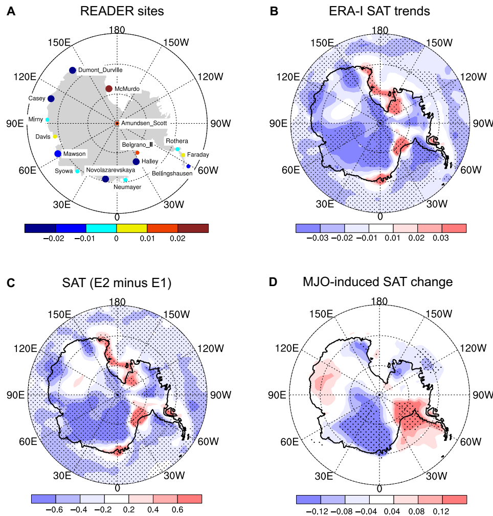
Fig. 1. Changes in the Antarctic SAT in austral summer (DJF) from 1979 to 2014. Antarctic SAT trends ( K\ year^{-1} ) based on (A) station observations and (B) ERA-I. (C) Differences in SAT (K) between the two epochs of 1997–2014 (E2) and 1979–1996 (E1). (D) SAT changes (E2 minus E1) induced by MJO-related variability estimated by the diagnostic equation, which incorporates the effects of decadal changes in MJO occurrence frequency with the intraseasonal SAT anomaly associated with the MJO (Eq. 1 in Materials and Methods). A large circle in (A) and stippling in (B) to (D) mark the regions with statistically significant changes at the 95% confidence level using the Mann-Kendall test [for the trend test in (A) and (B)], the Wilcoxon-Mann-Whitney test [for (C)], and the Monte Carlo method [for (D)], in which E1 and E2 years were randomly assigned and repeated 1000 times.
