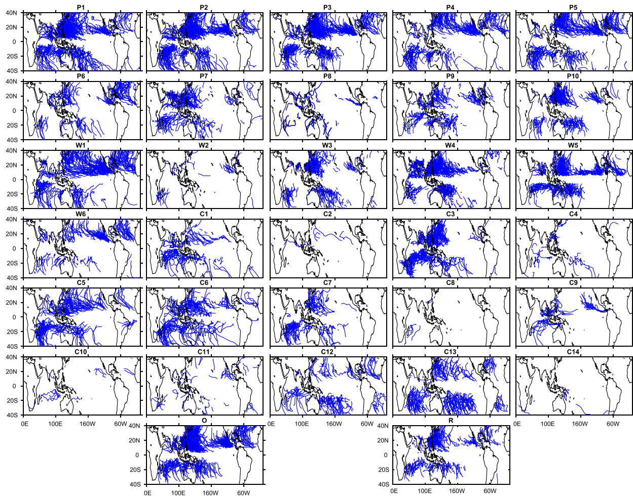
FIG. 2. Five years of tracks of TC-like storms in models (P1–P10, W1–W6, C1–C14), reanalysis ( R ), and observations ( O ). Data for the years 1991–95 were used for reanalysis, observations, and models C1–C14 and P1–P10, if available. In the case of W1–W6 the first five consecutive years were considered.
