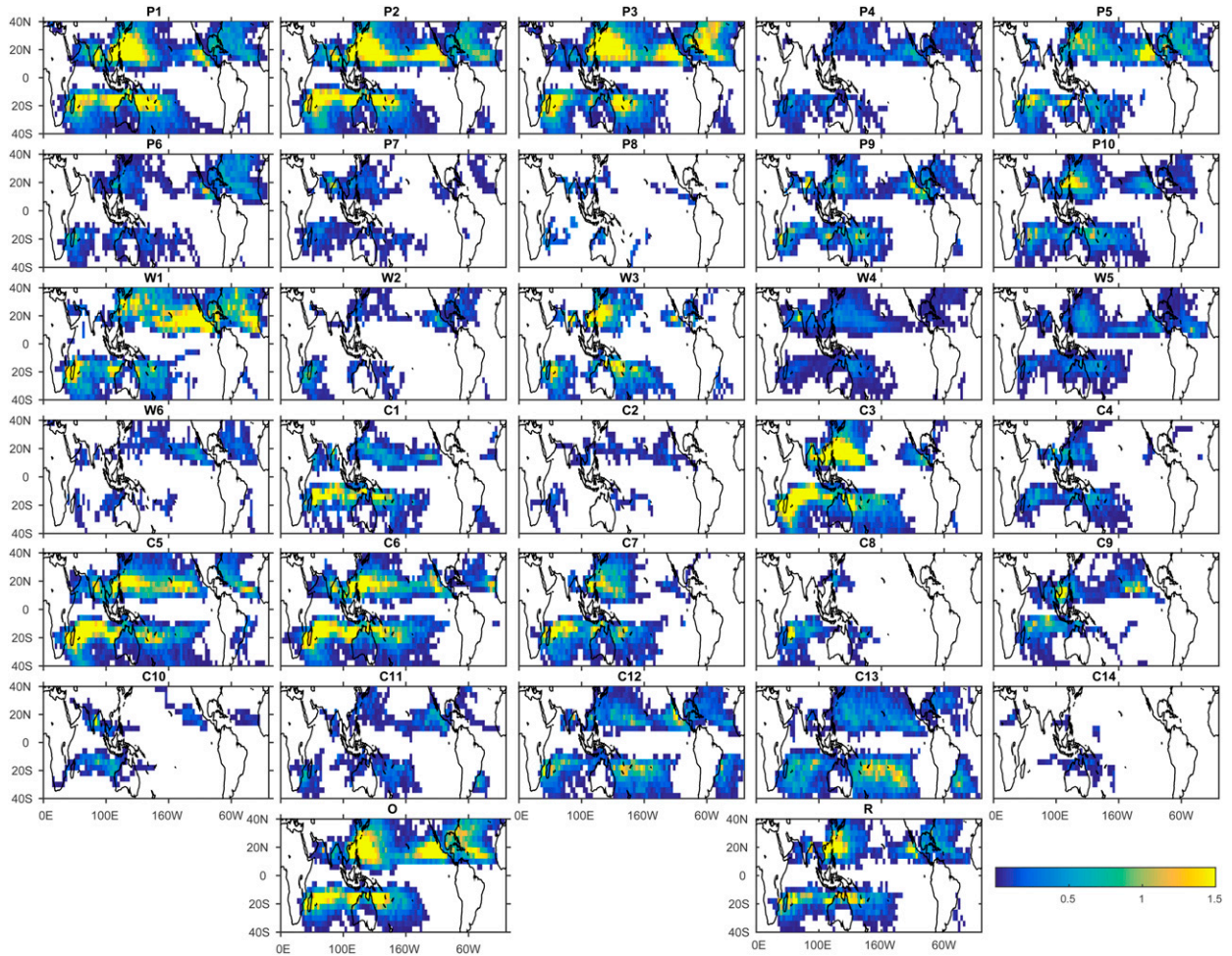
FIG. 3. Track density (mean of track passages per grid point) of TC storms in models (P1–P10, W1–W6, C1–C14), reanalysis ( R ), and observations ( O ) using all years available for each model (as shown in Tables 1–3). A common uniform grid of 4^\circ was used and normalized by the number of years available in each case.
